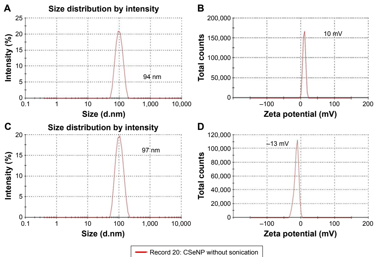
Figure 9 The average hydrodynamic diameter of (A) BSeNPs and (C) CSeNPs and the zeta potential of (B) BSeNPs and (D) CSeNPs.
