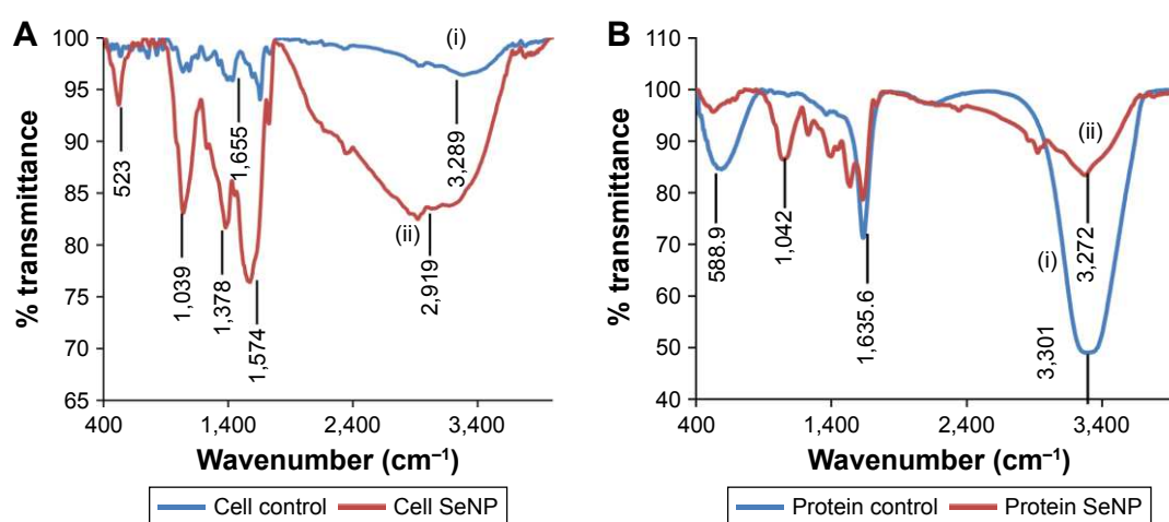
Figure 6 FTIR analysis of (A) cell suspension of Acinetobacter sp. SW30 and (B) TCP of Acinetobacter sp. SW30 (i) without \text{Na}_2\text{SeO}_3 and (ii) with \text{Na}_2\text{SeO}_3 . Abbreviations: FTIR, Fourier transform infrared spectroscopy; TCP, total cell protein.
